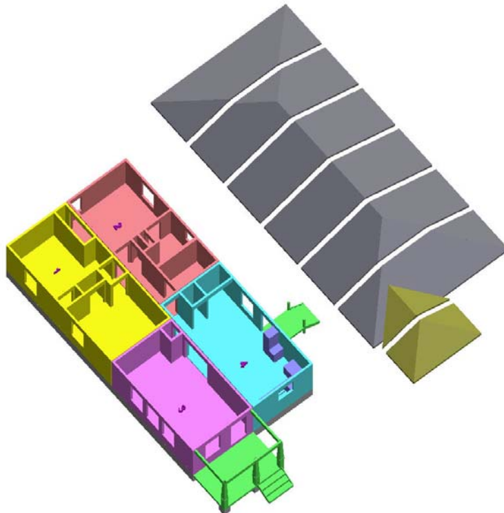
Exploded View of the 4-part modular house and roof segments (all to be student-fabricated in the Academy's shop)
